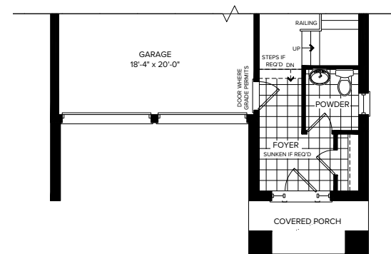
PARTIAL GROUND FLOOR ELEVATION C
