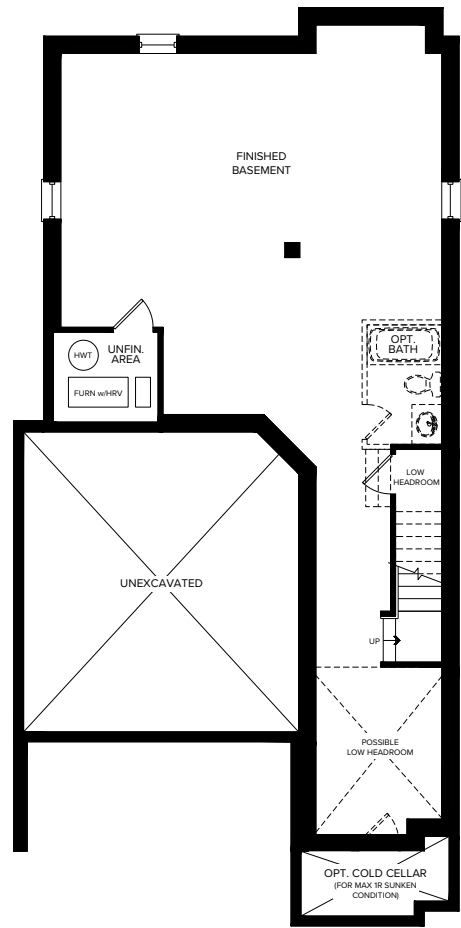
PARTIAL FINISHED BASEMENT ELEVATION B & C
