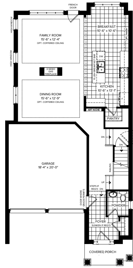
PARTIAL GROUND FLOOR ELEVATION B
