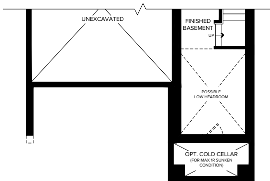
PARTIAL FINISHED BASEMENT ELEVATION B & C
