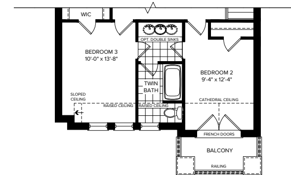
PARTIAL SECOND FLOOR ELEVATION B
