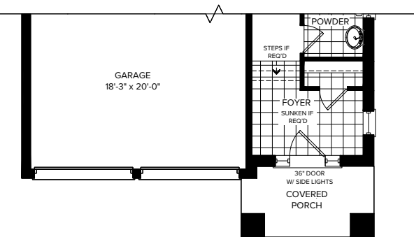
PARTIAL GROUND FLOOR ELEVATION C
