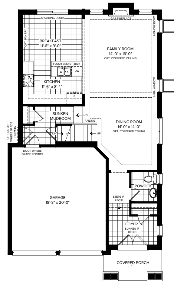
PARTIAL GROUND FLOOR ELEVATION B
