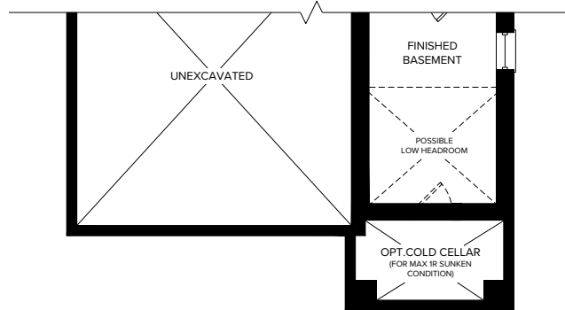
PARTIAL FINISHED BASEMENT ELEVATION C
