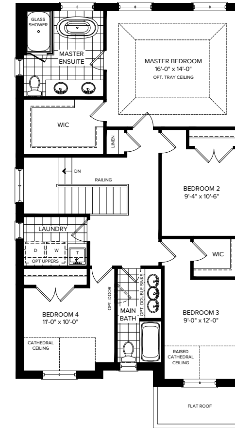
PARTIAL SECOND FLOOR ELEVATION B
