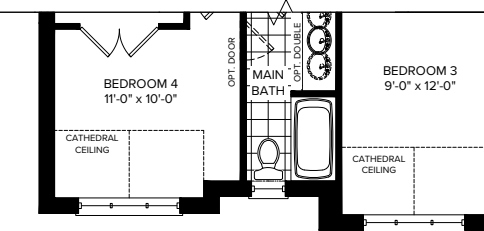
PARTIAL SECOND FLOOR ELEVATION B
