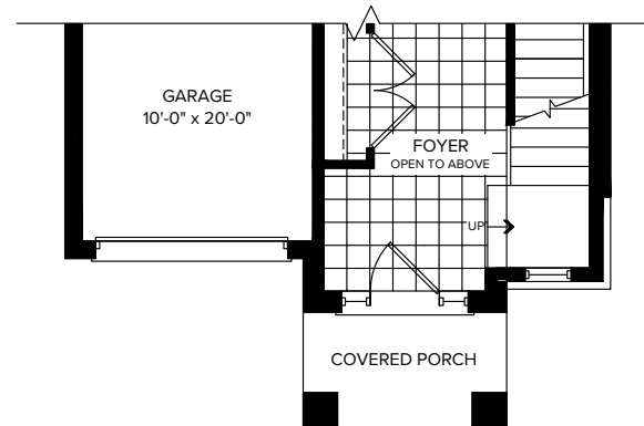
PARTIAL GROUND FLOOR ELEVATION C
