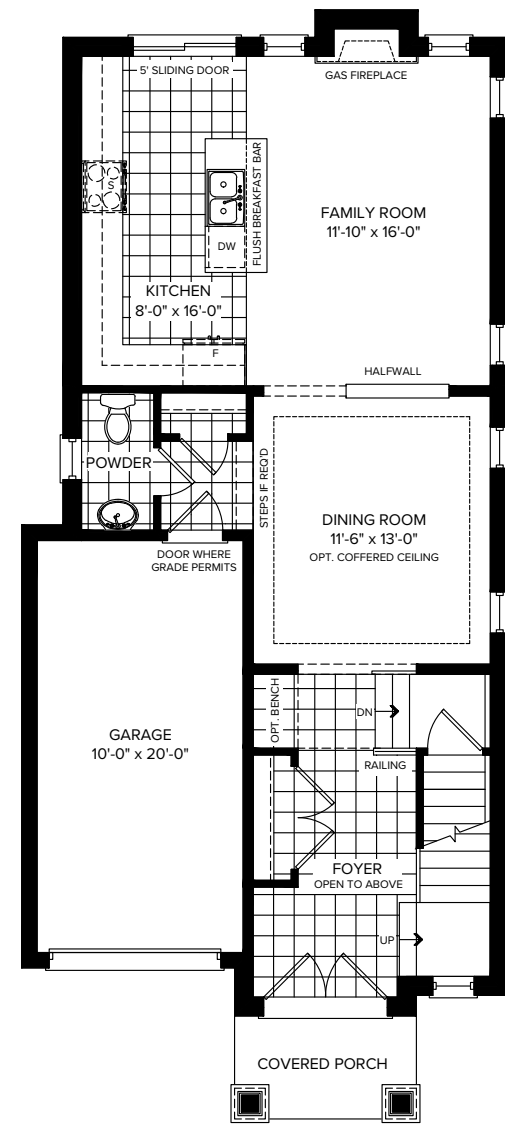
GROUND FLOOR ELEVATION A & B
