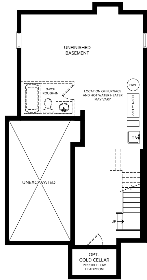
PARTIAL BASEMENT ELEVATION B
