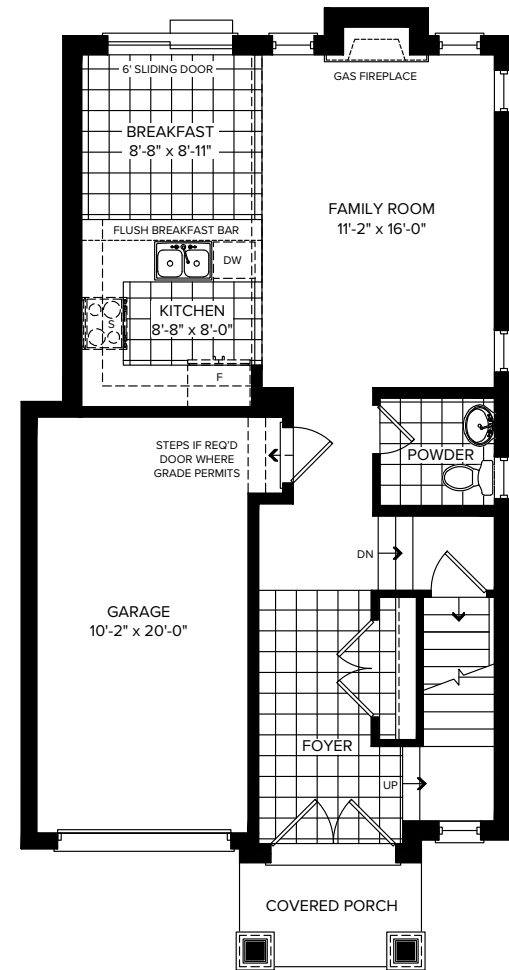
PARTIAL GROUND FLOOR ELEVATION B
