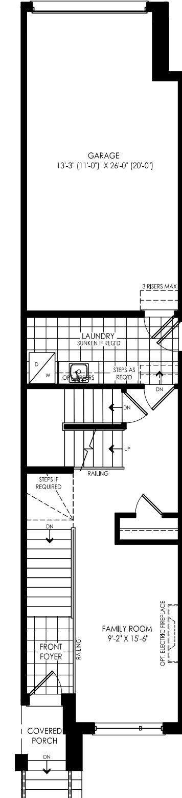
GROUND FLOOR PLAN ELEV. 'A'
