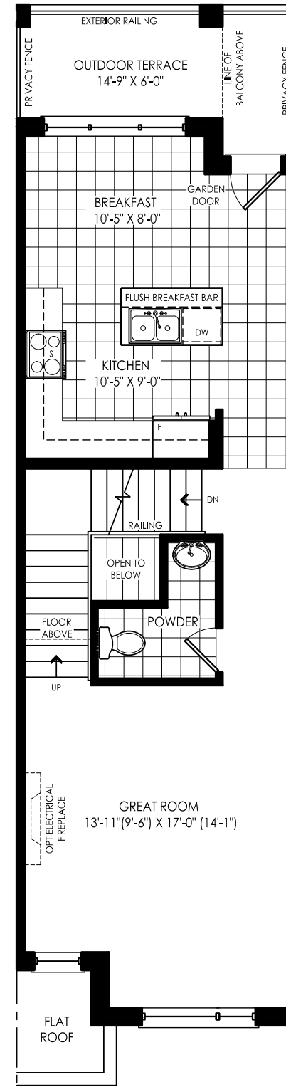
SECOND FLOOR PLAN ELEV. 'A'
