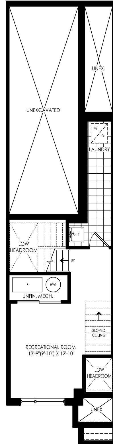
OPT. FINISHED BASEMENT PLAN ELEV. 'A'
