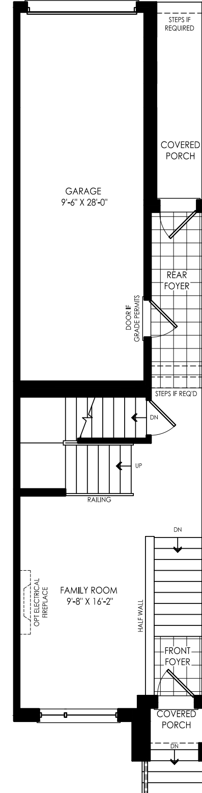
GROUND FLOOR PLAN ELEV. 'A'
