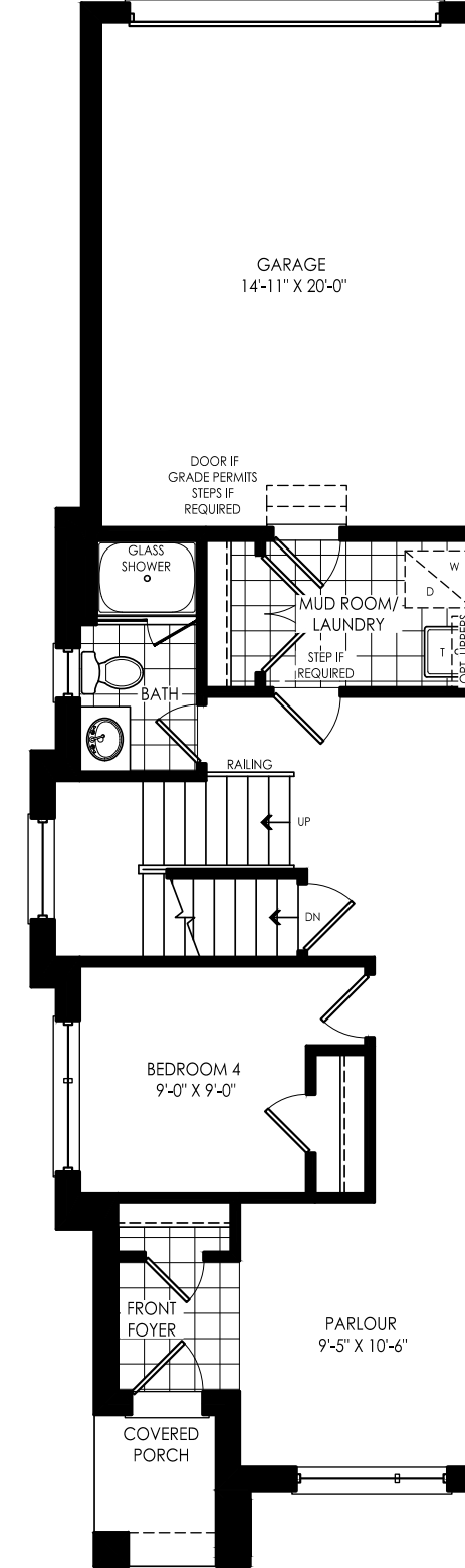
OPT. GROUND FLOOR PLAN ELEV. 'A'
