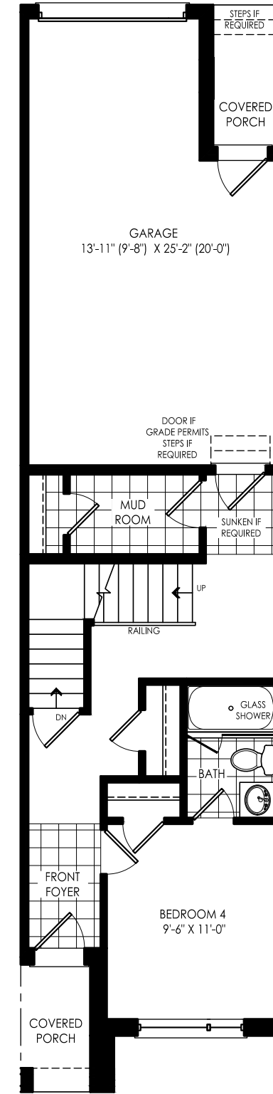
OPT. GROUND FLOOR PLAN ELEV. 'A'
