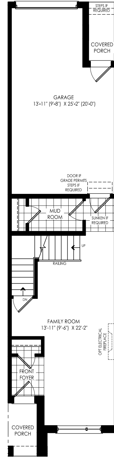
GROUND FLOOR PLAN ELEV. 'A'
