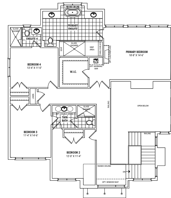
SECOND FLOOR PLAN ELEVATION D
