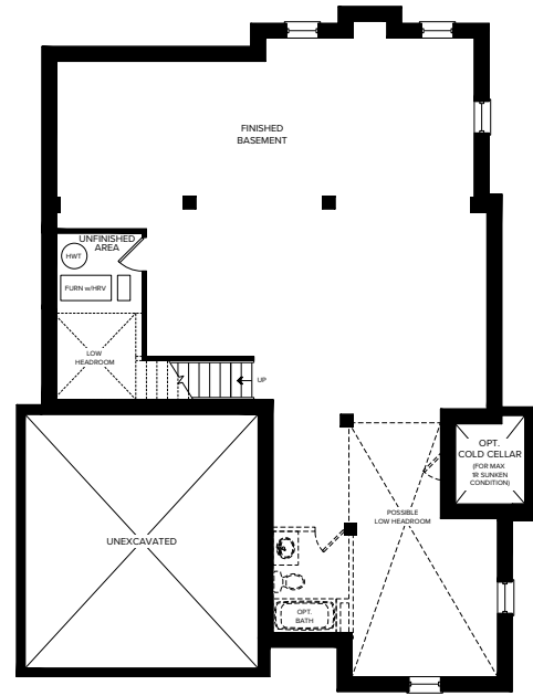
FINISHED BASEMENT ELEVATION C
