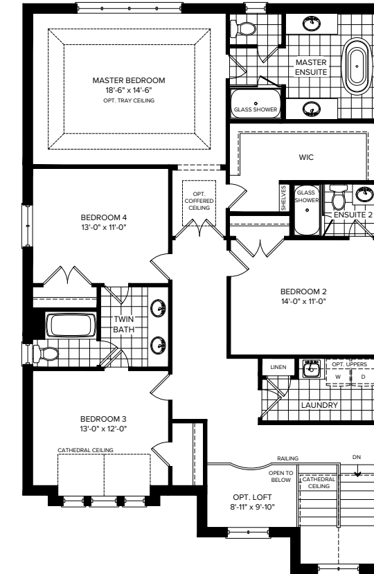
PARTIAL SECOND FLOOR ELEVATION B
