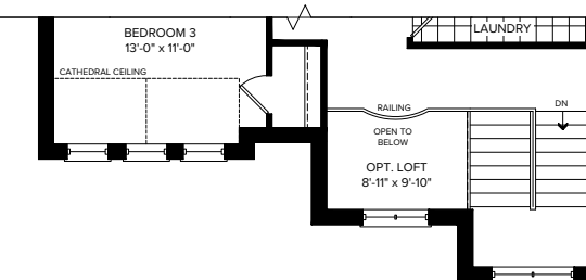
PARTIAL SECOND FLOOR ELEVATION B
