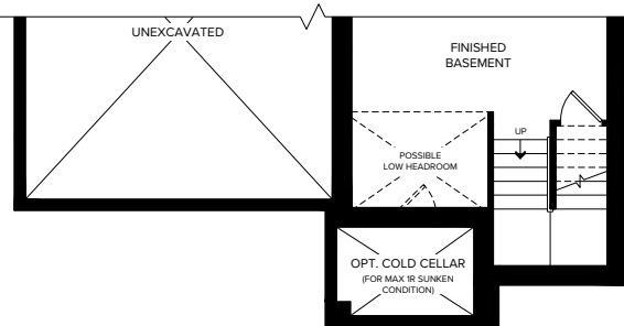
PARTIAL FINISHED BASEMENT ELEVATION B
