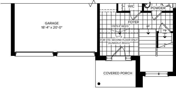
PARTIAL GROUND FLOOR ELEVATION C
