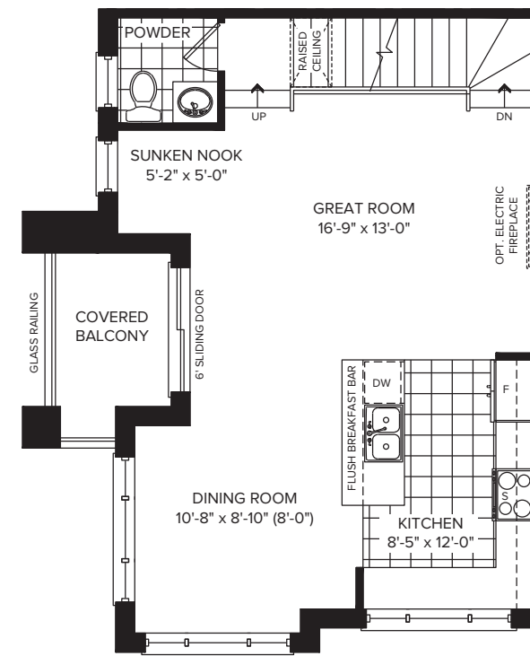
THIRD FLOOR ELEVATION B1
