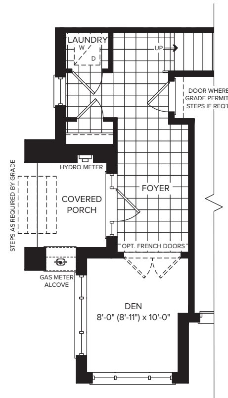
PARTIAL GROUND FLOOR ELEVATION B2
