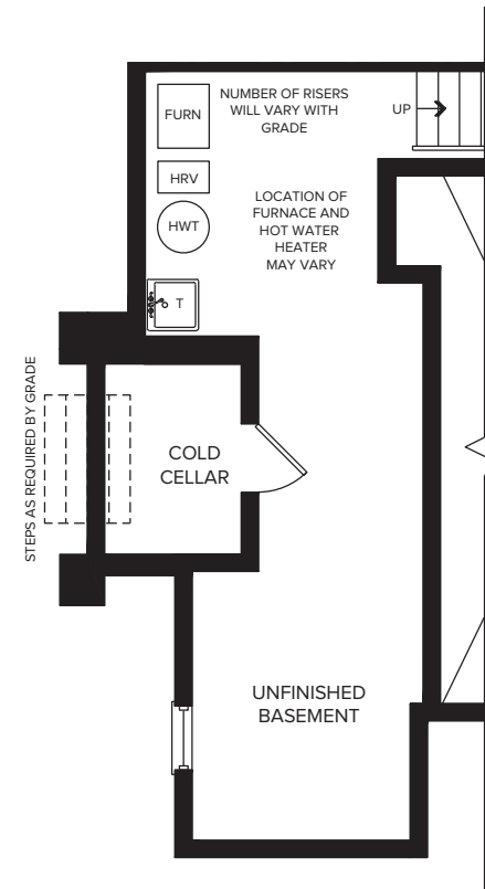
PARTIAL BASEMENT ELEVATION B2
