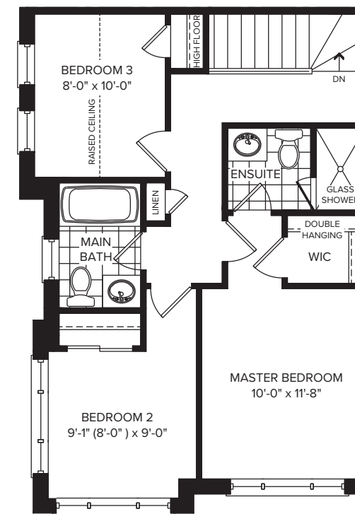
THIRD FLOOR ELEVATION B1
