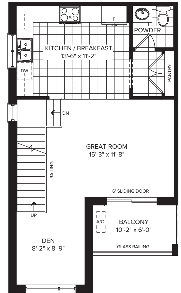
MAIN FLOOR ELEVATION A
