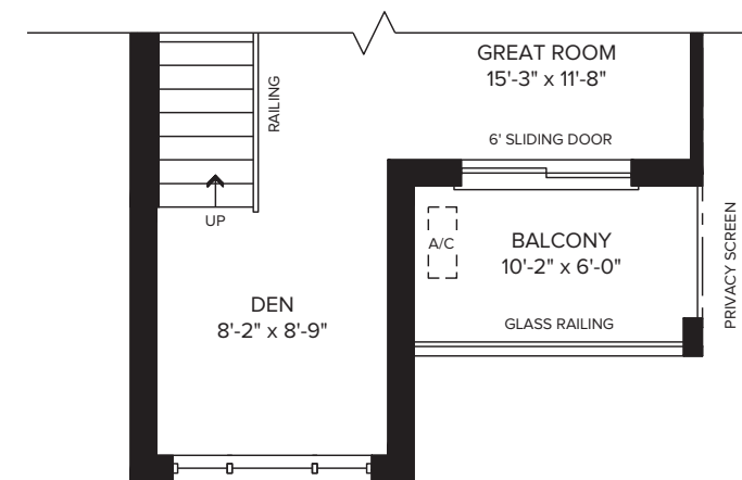
PARTIAL MAIN FLOOR ELEVATION B
