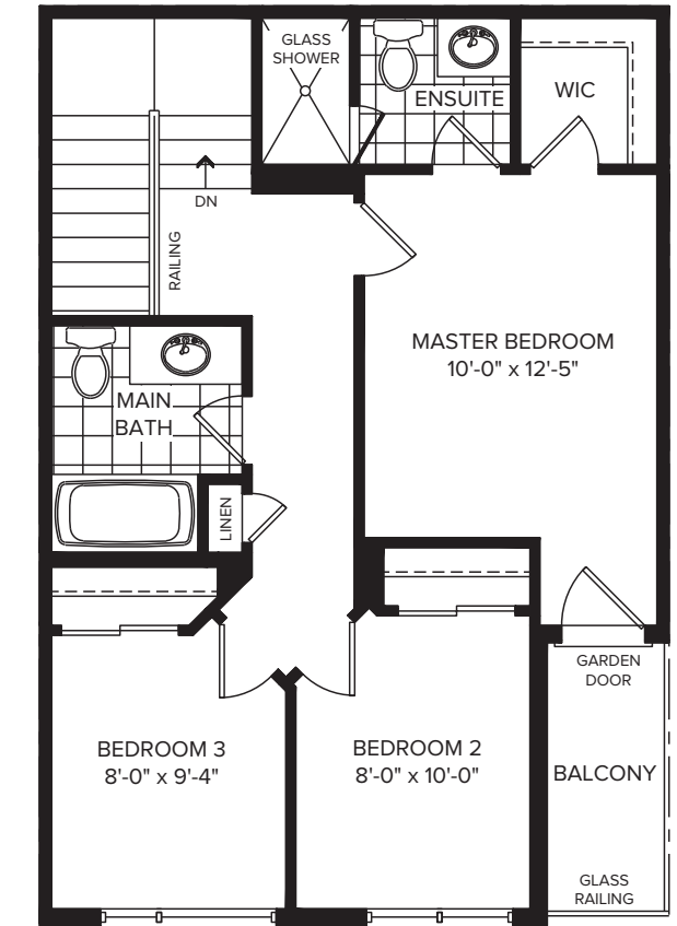
THIRD FLOOR ELEVATION A
