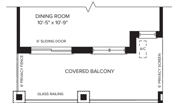
PARTIAL MAIN FLOOR ELEVATION B
